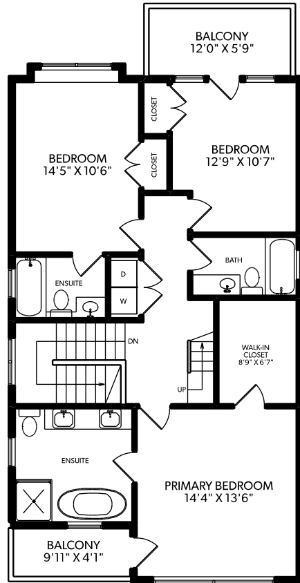
UPPER FLOOR
